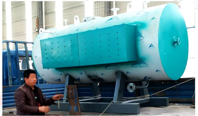
2014.10 河南荥阳起升建材有限公司2t电蒸汽锅炉 2014.10 2t/h electric steam boiler in Henan Qisheng Construction Materials Co.,Ltd
